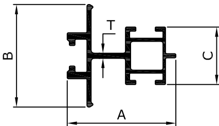
CEILING GRID SECTION (VCR)
