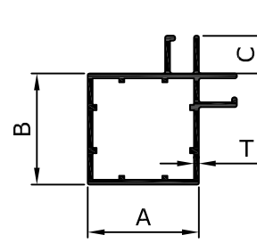
KITCHEN FRAME SECTION (VKD)
