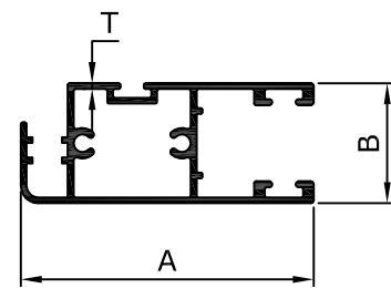
INDUSTRIAL SECTION (VMM)
