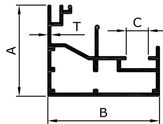
INDUSTRIAL SECTION (VIS)
