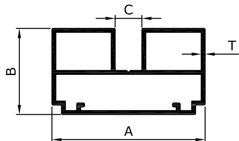
INDUSTRIAL SECTION (VIS)
