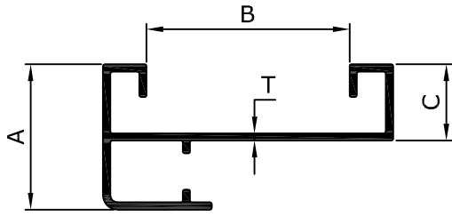
INDUSTRIAL SECTION (VIS)
