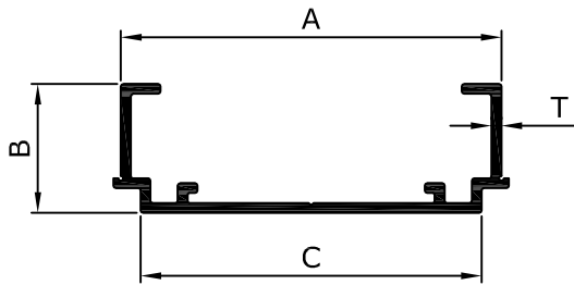
INDUSTRIAL SECTION (VIS)
