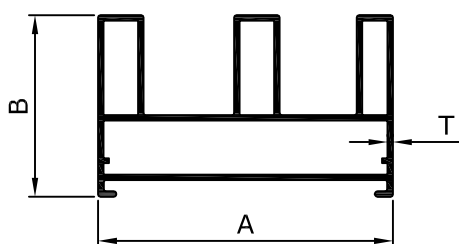
INDUSTRIAL SECTION (V3T)
