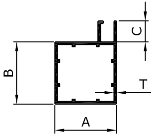
KITCHEN FRAME SECTION (VKS)
