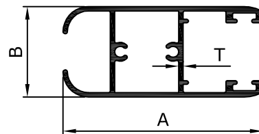
INDUSTRIAL SECTION (VDS)
