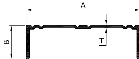
INDUSTRIAL SECTION (VLD)
