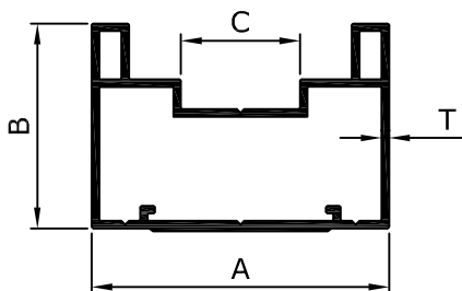
INDUSTRIAL SECTION (VIS)
