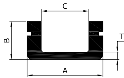
PANEL BOARD SECTION (VIS)
