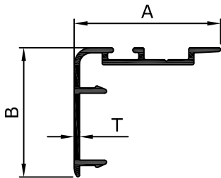
INDUSTRIAL SECTION (VDS)
