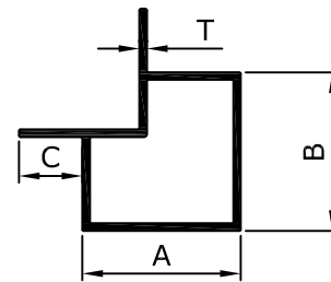
CORNER SECTION (VCR)
