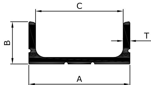
PANEL BOARD SECTION (VIS)
